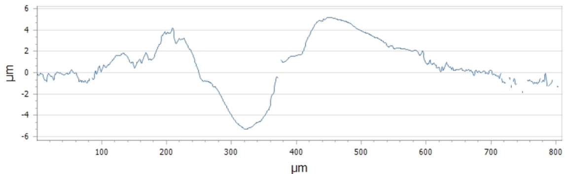
Figure 54. Depth profile of crater from 10 shots. \lambda = 2947 \text{ nm} , \tau_p = 60.23 \mu\text{s} , \omega_0 \approx 307 \mu\text{m} , F = 250 \text{ J/cm}^2 , Material: Al, P = 1 \text{ atm} , T = 300 \text{ K} .
