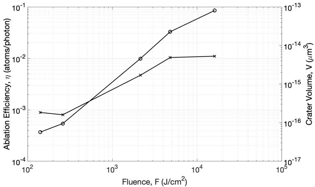
Figure 19. Ablation efficiency (×, left axis) and crater volume (o, right axis). \lambda = 1064 \text{ nm} , \tau_p = 1 \text{ } \mu\text{s} , \omega_0 \approx 10 \text{ } \mu\text{m} , F : varied, Material: Ge, P = 1 \text{ atm} , T = 300 \text{ K} .
