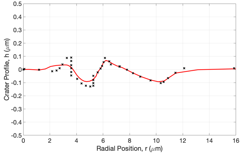
Figure 43. Simulated (red) and measured (×) craters. \lambda = 1064 nm, \tau_p = 28 \mu s, \omega_0 \approx 6.7 \mu m, F = 22.1 J/cm 2 , Material: Si, P = 1 atm, T = 300 K.
