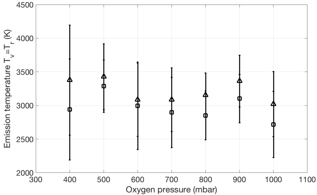
Figure 58. Temperature from (□) optically thick fit of entire observed AIO B-X spectra and (Δ) optically thin fit of \Delta v = -1 sequence. \lambda = 2947 nm, \tau_p = 60.23 \mu\text{s} , \omega_0 \approx 307 \mu\text{m} , F = 250 J/cm 2 , Material: Al, P : varied, T = 300 K.
