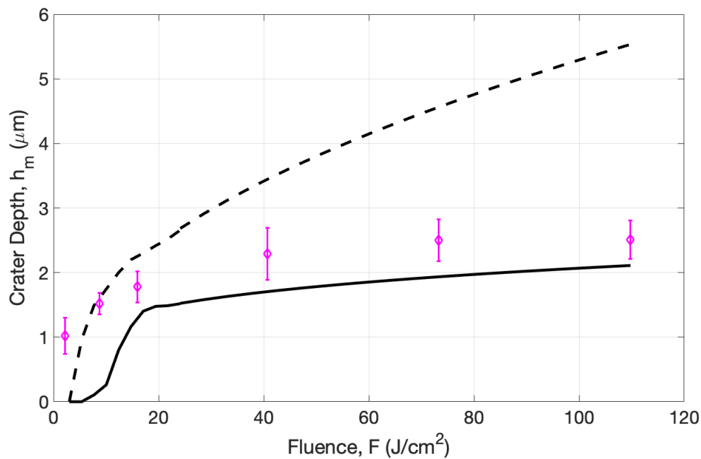
Figure 45. Simulated crater depths using (dashed line) TEM 00 and (solid line) TEM 40 modes, and (◇) measured crater depth, h_m . \lambda = 1064 nm, \tau_p = 28 \mu s, \omega_0 \approx 6.7 \mu m, F : varied, Material: Ge, P = 1 atm, T = 300 K.
