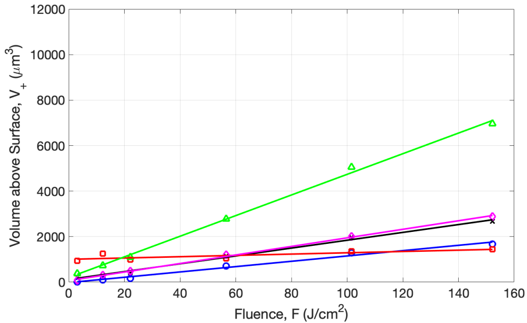
Figure 30. Measured crater volume above surface, V_+ . \lambda = 1064 \text{ nm} , \tau_p = 28 \mu\text{s} , \omega_0 \approx 6.7 \mu\text{m} , F : varied, Material: Al ( \times ), Si ( \circ ), Ti ( \square ), Ge ( \diamond ), InSb ( \triangle ), P = 1 \text{ atm} , T = 300 \text{ K} .
