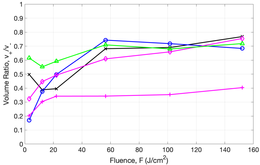
Figure 39. Volume ratio, V_+/V_- . \lambda = 1064 nm, \tau_p = 28 \mu s, \omega_0 \approx 6.7 \mu m, F : varied, Material: Al ( \times ), Si ( \circ ), Ge ( \diamond , + ), InSb ( \triangle ), P = 1 atm and ( + ) P = 2.2 \times 10^{-3} atm, T = 300 K.
