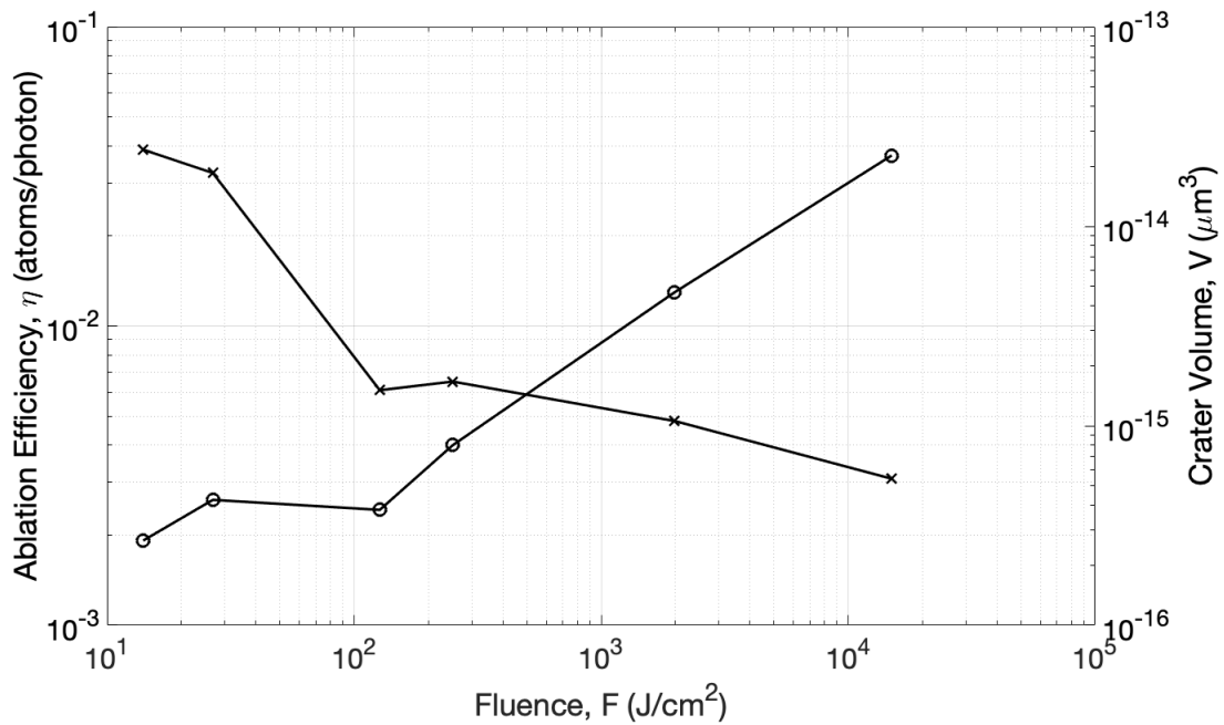
Figure 18. Ablation efficiency (×, left axis) and crater volume (o, right axis). \lambda = 1064 \text{ nm} , \tau_p = 10 \text{ ns} , \omega_0 \approx 10 \text{ } \mu\text{m} , F : varied, Material: Ge, P = 1 \text{ atm} , T = 300 \text{ K} .
