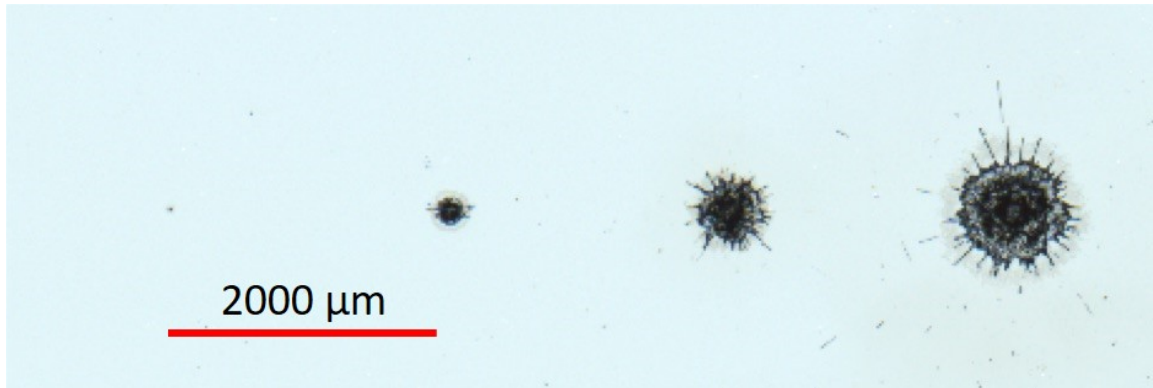
Figure 4. Craters from laser ablation in the melt flow regime. \lambda = 1064 \text{ nm} , \tau_p = 1 \text{ } \mu\text{s} , \omega_0 \approx 10 \text{ } \mu\text{m} , F : varied, Material: Si, P = 1 \text{ atm} , T = 300 \text{ K} .
