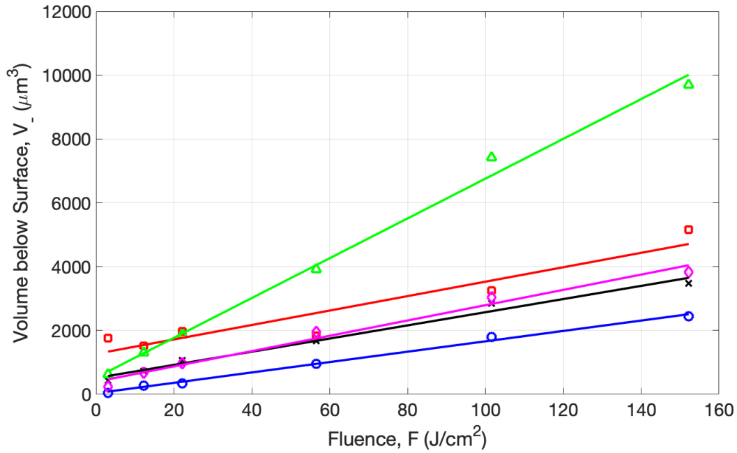
Figure 29. Measured crater volume below surface, V_- . \lambda = 1064 \text{ nm} , \tau_p = 28 \mu\text{s} , \omega_0 \approx 6.7 \mu\text{m} , F : varied, Material: Al ( \times ), Si ( \circ ), Ti ( \square ), Ge ( \diamond ), InSb ( \triangle ), P = 1 \text{ atm} , T = 300 \text{ K} .
