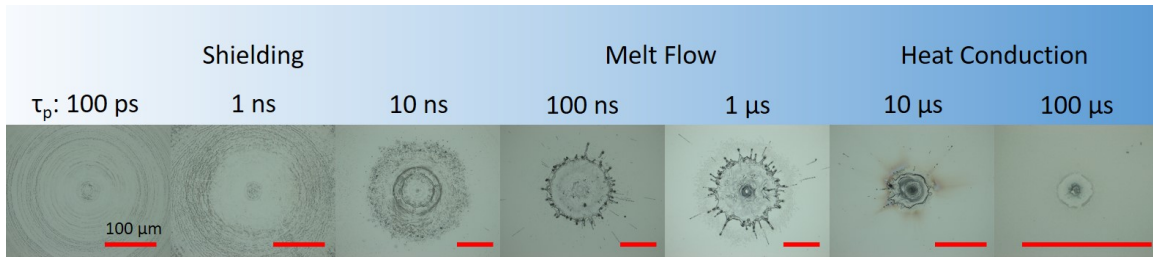
Figure 1. Examples of dominant phenomenological temporal regimes in laser ablation. \lambda = 1064 \text{ nm} , \tau_p : varied, \omega_0 \approx 10 \mu\text{m} , F \approx 15 \text{ kJ/cm}^2 , Material: Ge, P = 1 \text{ atm} , T = 300 \text{ K} . Red bars are 100 \mu\text{m} length in each image.
