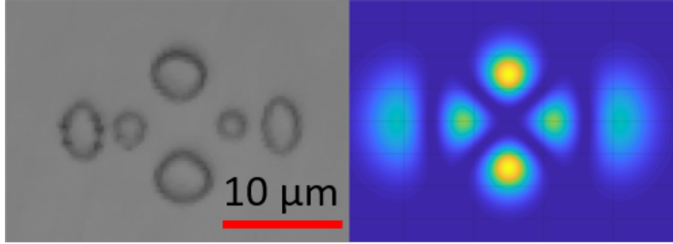
Figure 24. Measured crater (left) and simulated Gaussian TEM 40 and TEM 02 transverse spatial modes (right). \lambda = 1064 \text{ nm} , \tau_p = 28 \text{ } \mu\text{s} , \omega_0 \approx 6.7 \text{ } \mu\text{m} , F \approx 3.1 \text{ J/cm}^2 , Material: Si, P = 1 \text{ atm} , T = 300 \text{ K} .
